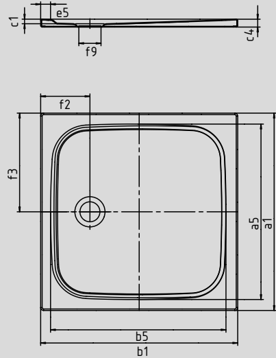
Model 2255 with low profile support
