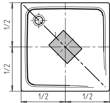
SUPERPLAN Mod. 391 1000x1000 Mod. 399 1200x1200
