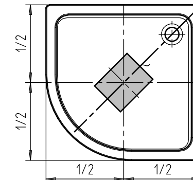
ARRONDO Mod. 872 1000x1000 Mod. 873 1000x1000
